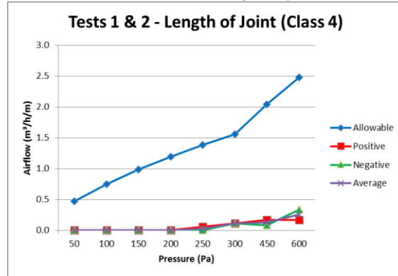
Graph 2 – Air Permeability – Length of joint
