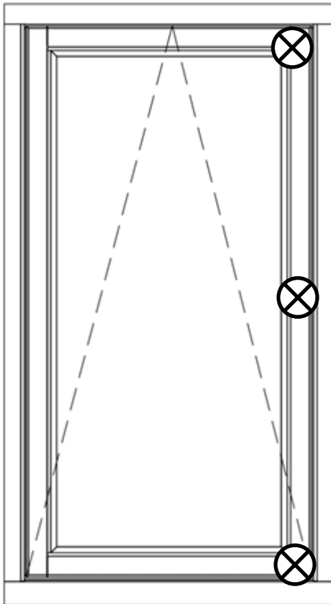
Figure 2 – Position of deflection measurement sensors
