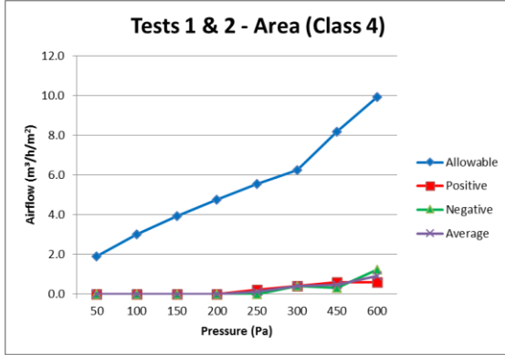
Graph 1 –Air Permeability - Area
