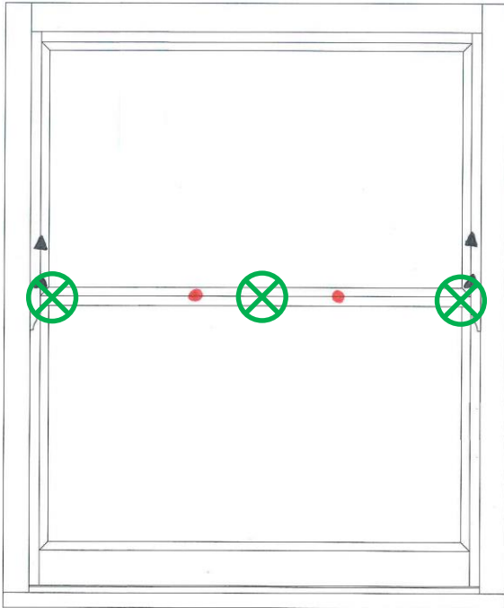
Figure 3 – Position of deflection measurement sensors
