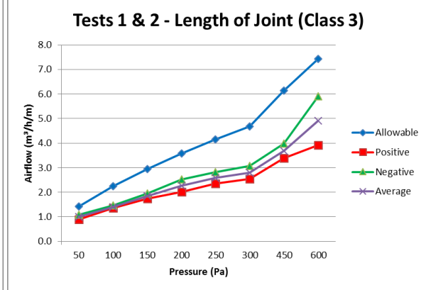
Graph 2 – Air Permeability – Length of joint
