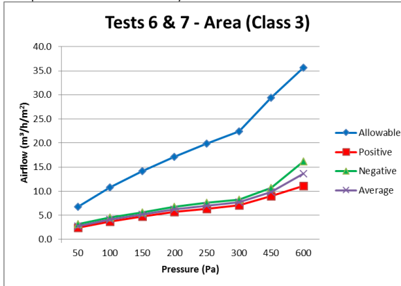
Graph 3 – Air Permeability - Area
