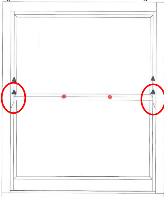
Figure 2 – Areas of concentrated air leakage
