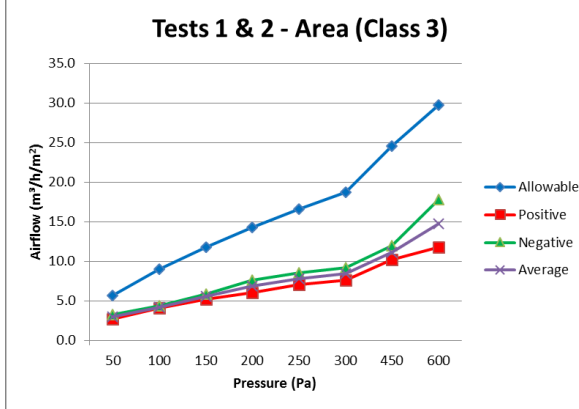
Graph 1 – Air Permeability - Area
