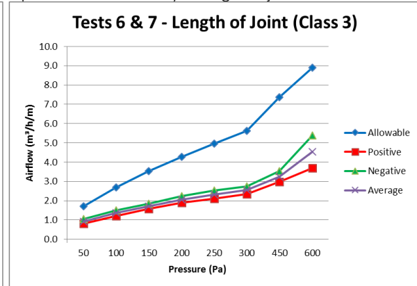
Graph 4 – Air Permeability – Length of joint
